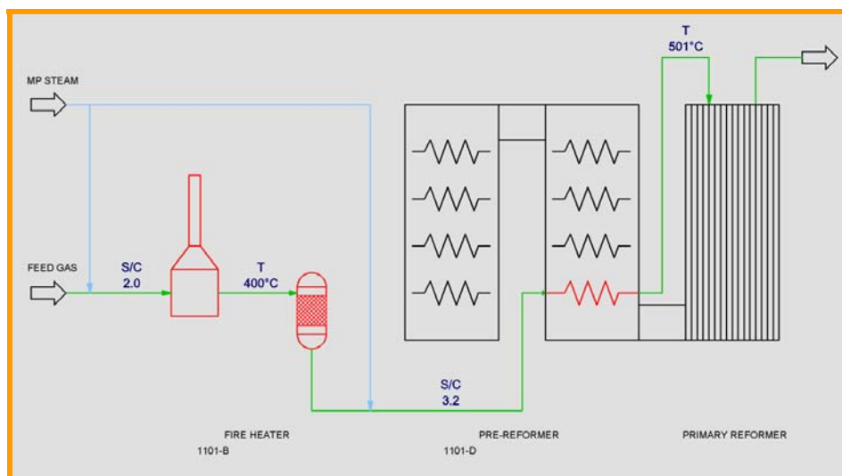
Fig. 6: New Fired Heater and Pre-Reformer
