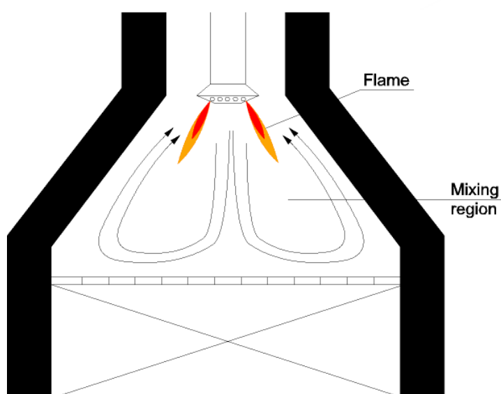
Fig. 3: Casale design for secondary reformer burner
