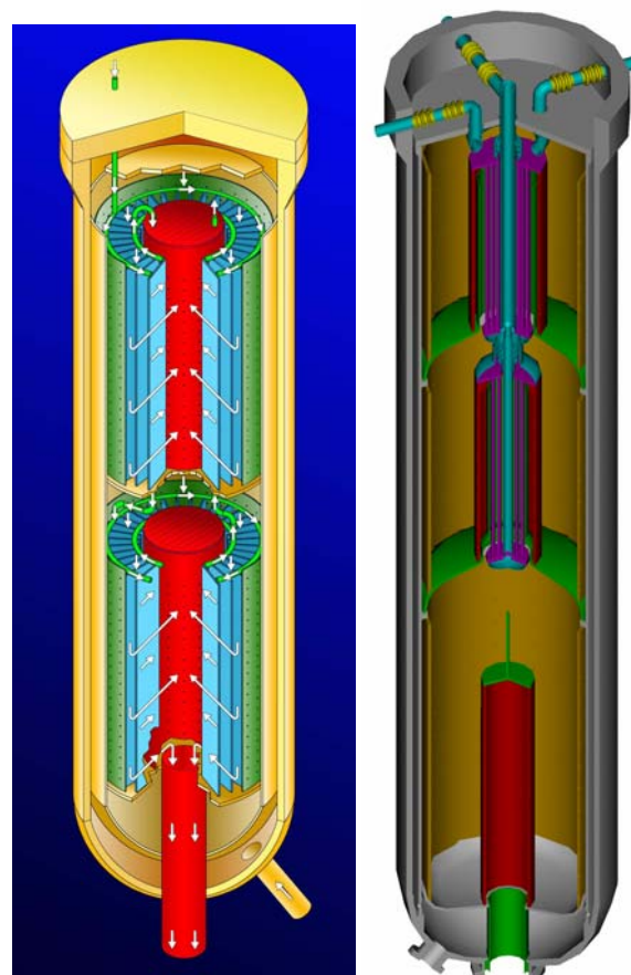
Fig. 2: Plate-cooled and 3-bed ammonia converter
