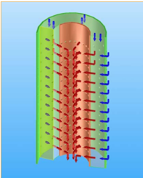
Fig. 1: Gas Distribution in an Axial-Radial Catalyst Bed
