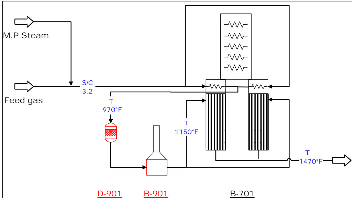
Fig. 8 - Pre-Reformer Arrangement, new items in red.
