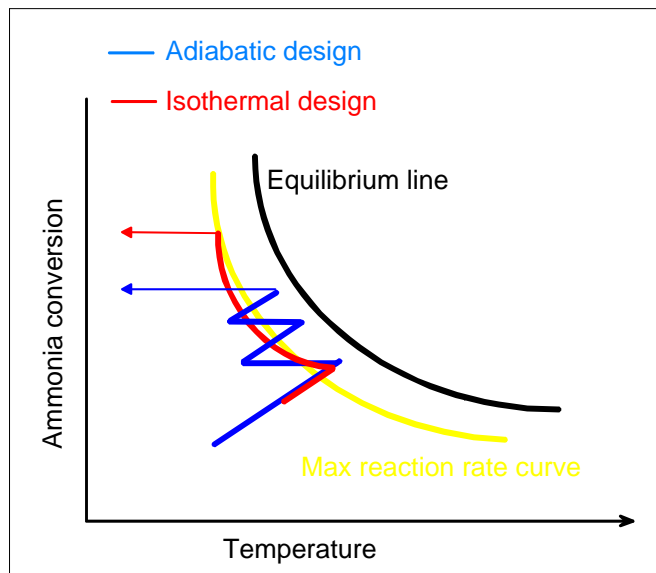
Fig. 9 - Temperature Profile of the IAC.
