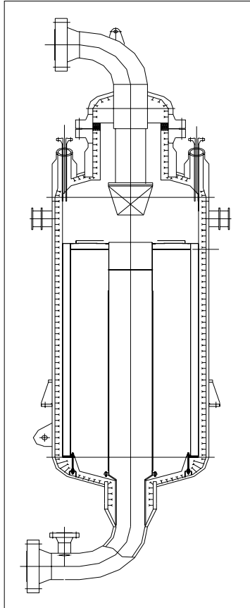
Fig. 7 - PCS Axial-Radial Pre-Reformer
